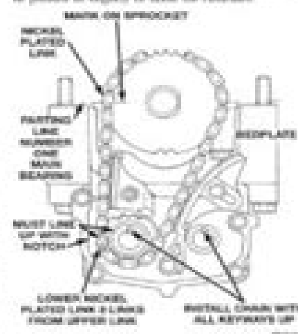
Fig. 42 Balance Shaft Timing
