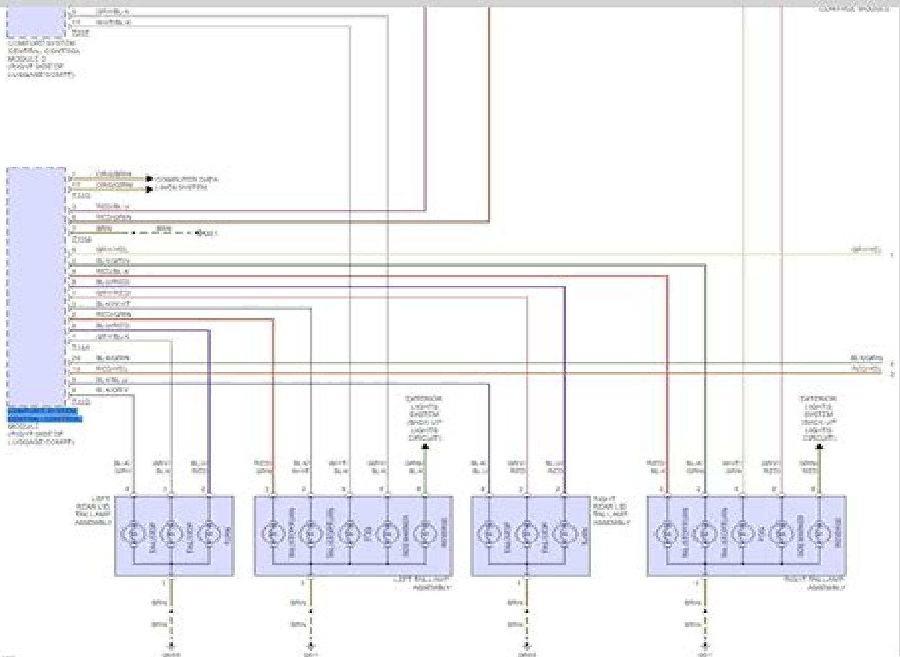
Fig 2: Exterior Lamps Circuit (1 of 2)
