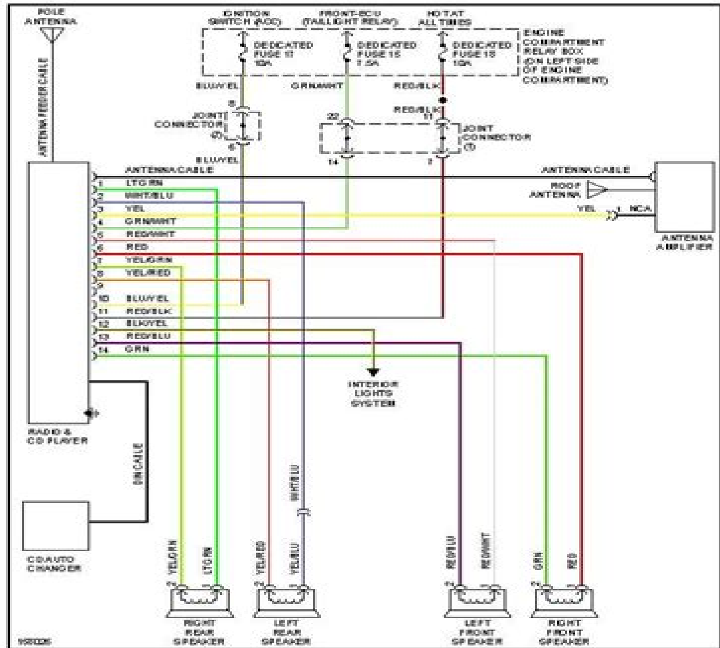
2002 Mitsubishi Lancer O-Z Rally-Fig. 31: Radio Circuits, 4 Speaker System
