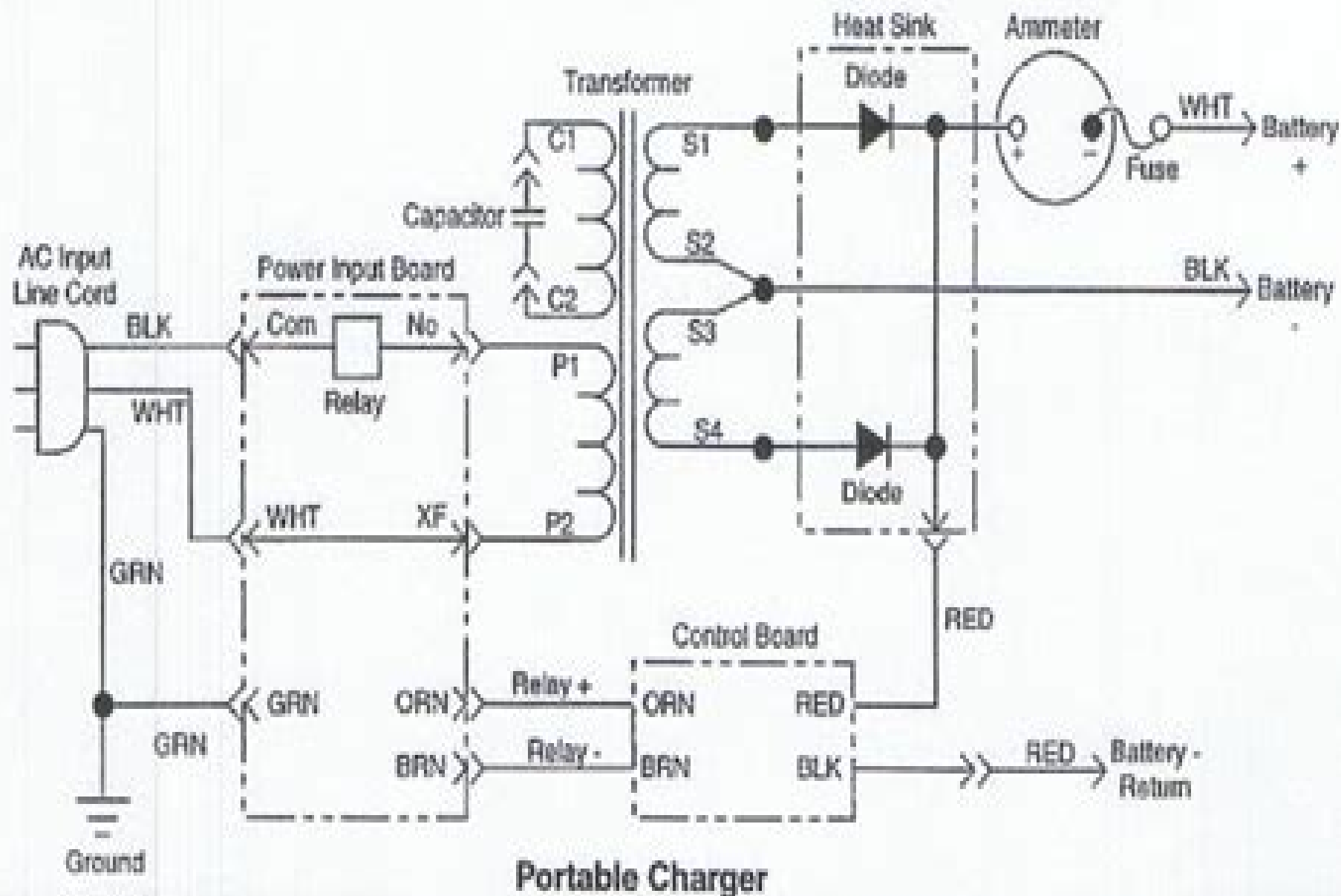
Fig. 5 PowerWise™ Charger Wiring Diagrams
