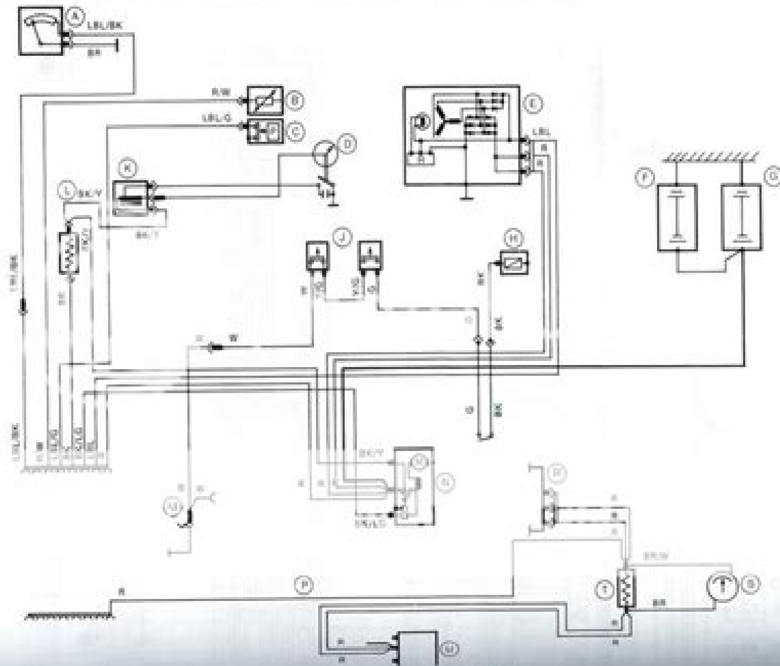
Fig. 13.32 Wiring diagram: interactive - all models
