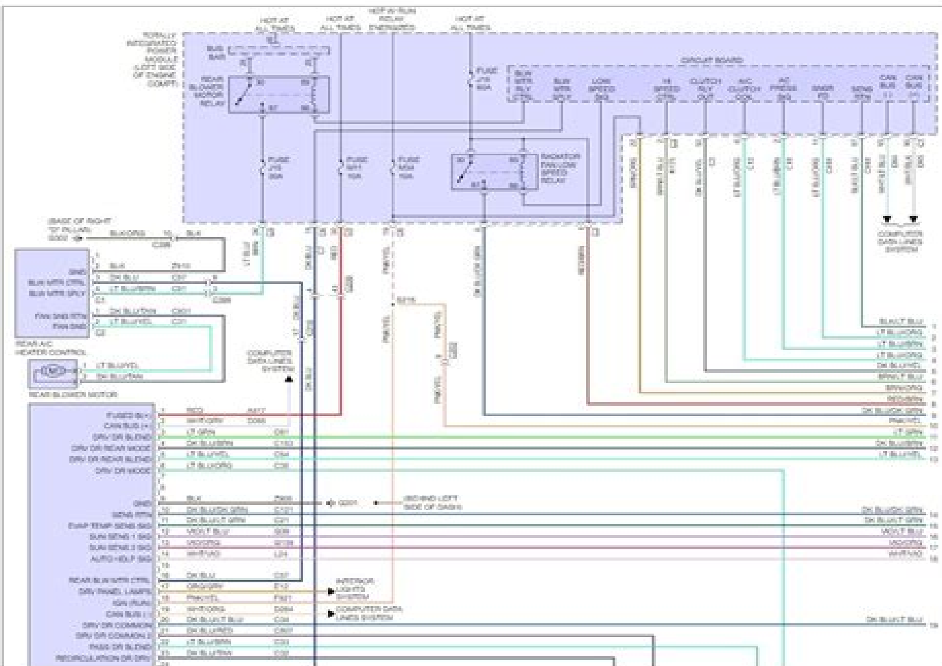
Fig 1: Automatic A/C Circuit (1 of 2)
