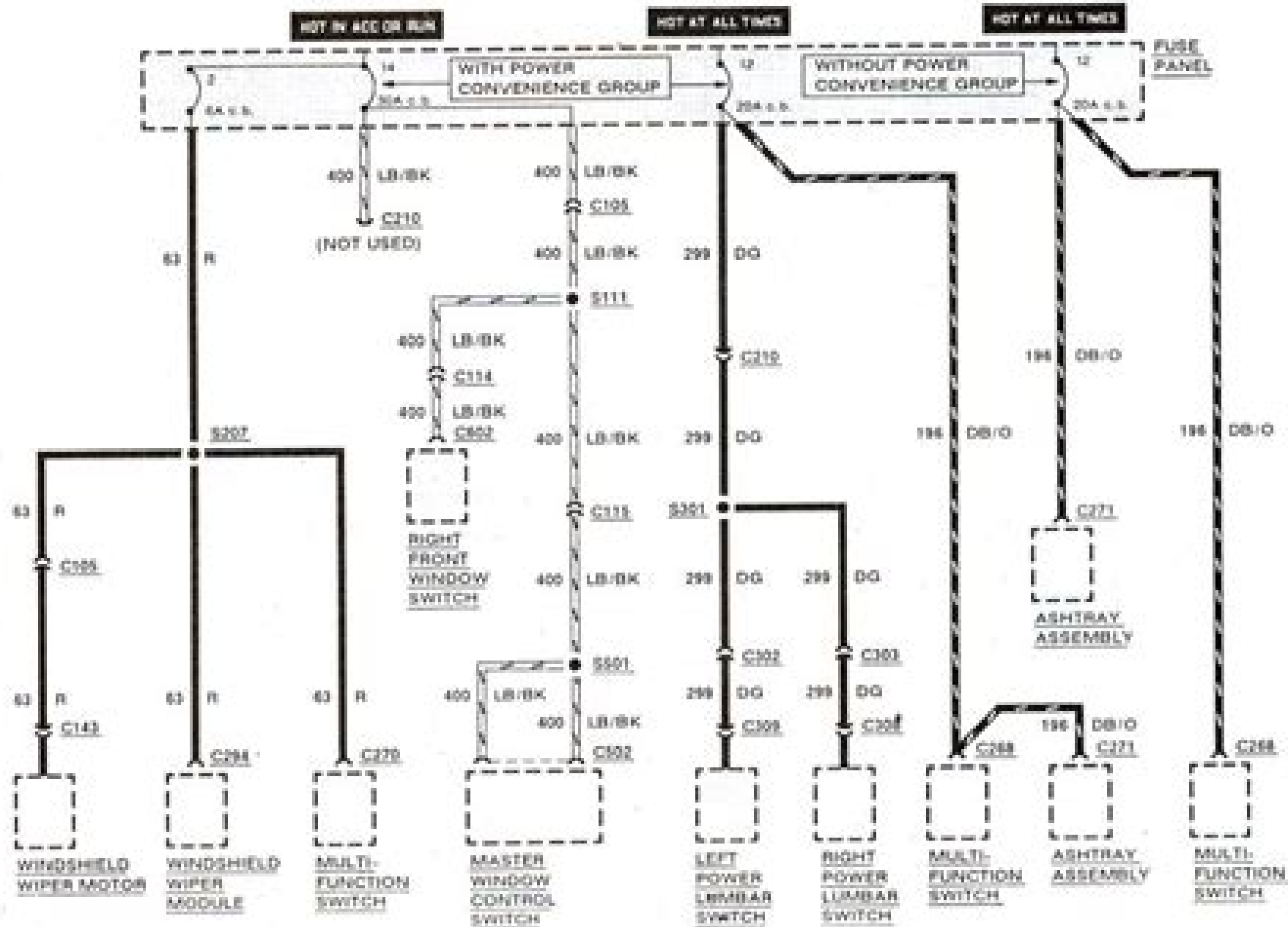
Power distribution – (typical – 1991 shown) (part 4 of 7)
