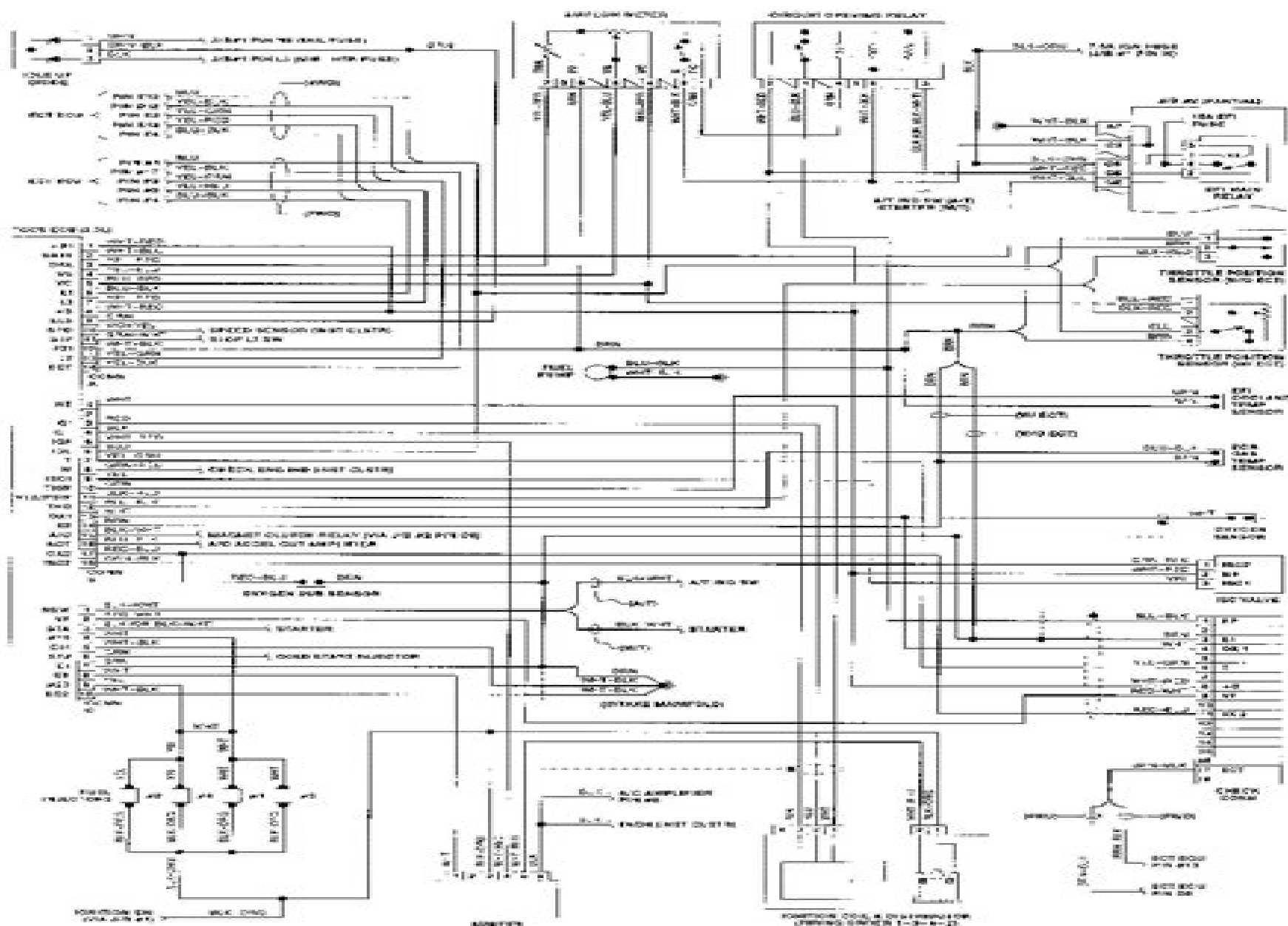
Fig. 1: Wiring Diagram (Camry 2.0L) 1991 Toyota Camry LE
