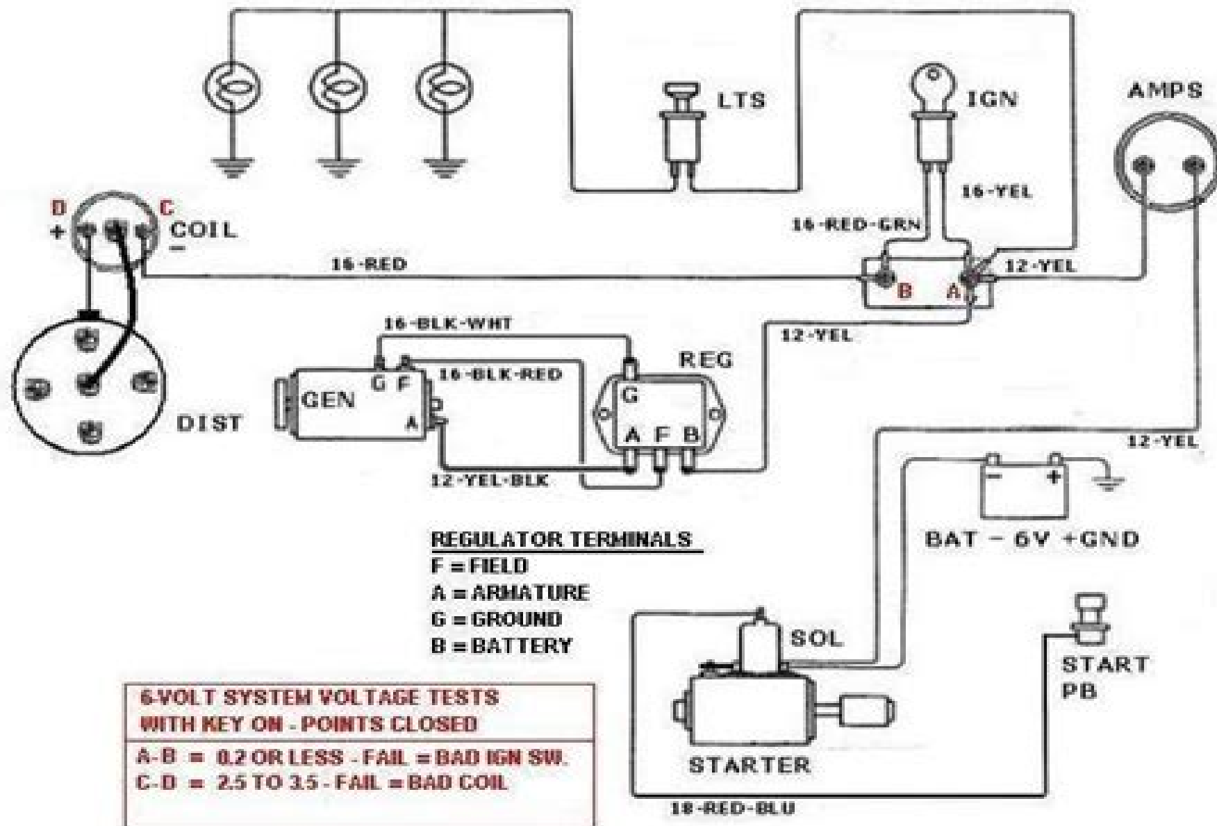
FORD 8N TRACTOR WIRING - SIDE DISTRIBUTOR 1950 TO 1953 Jubilee K.LaRue - Free of Charge - 2006
