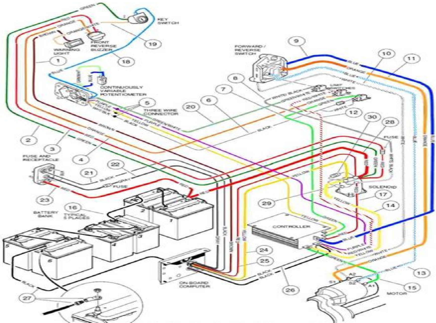
95-03 48 volt electric club car wiring diagram
