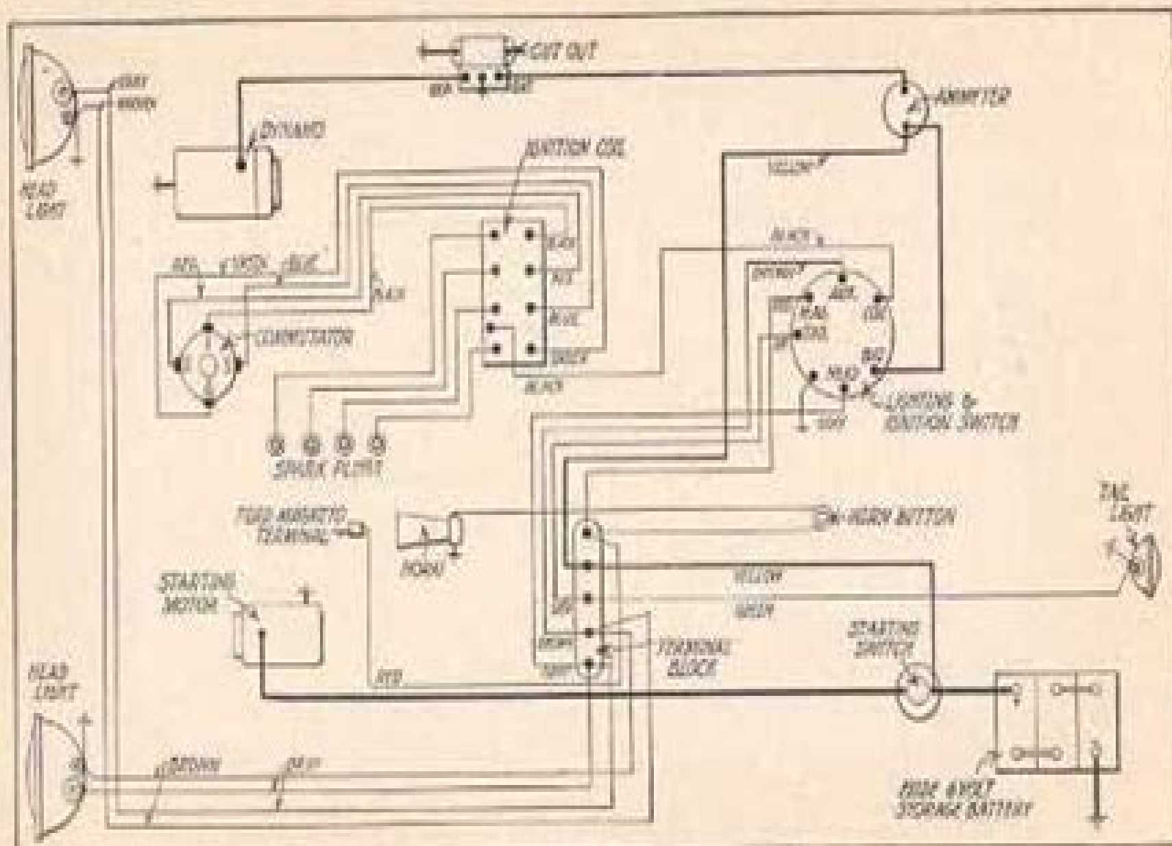
Fig. 17. Wiring Diagram with Cutout on Dash
