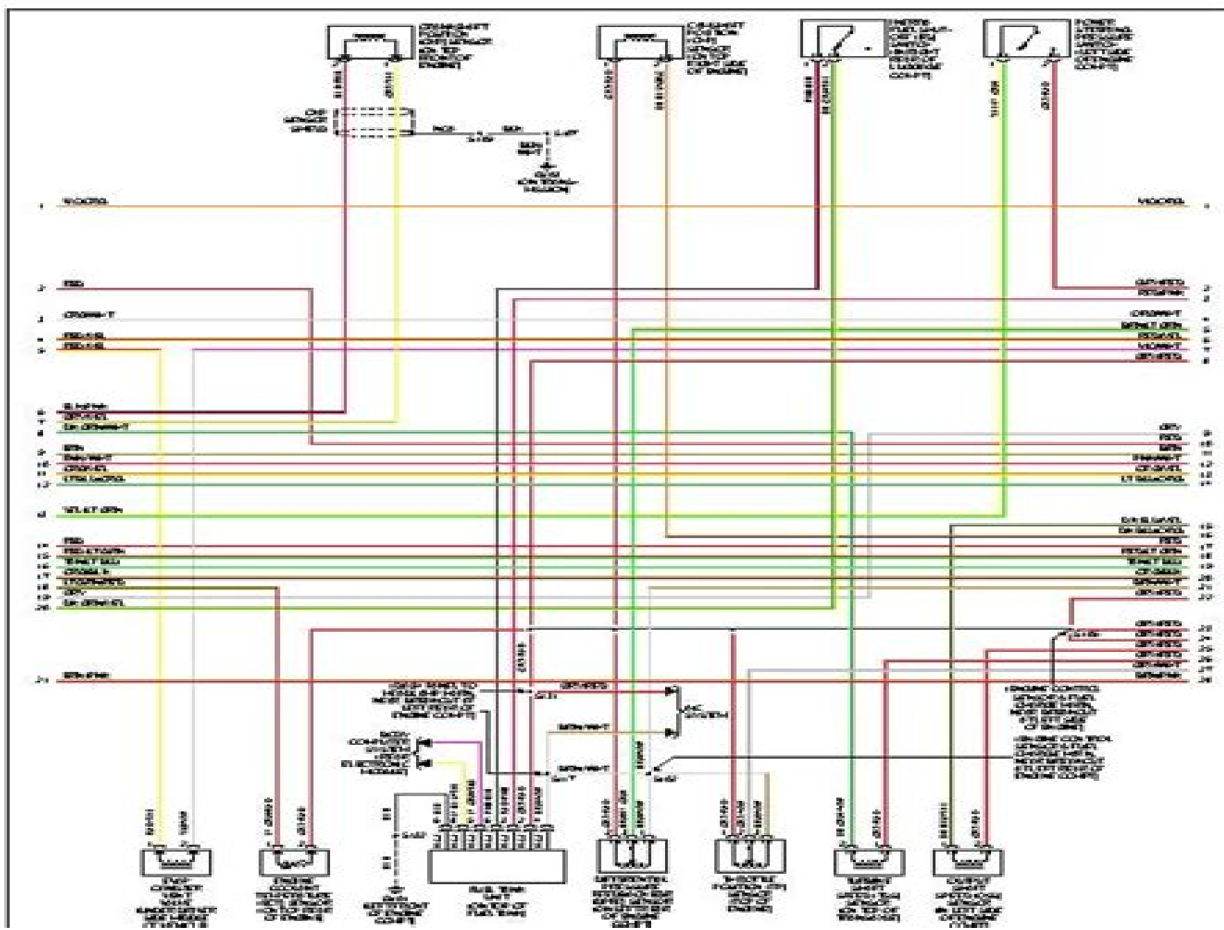
2002 Ford Windstar-Fig. 16: 3.8L, Engine Performance Circuits (2 of 4)
