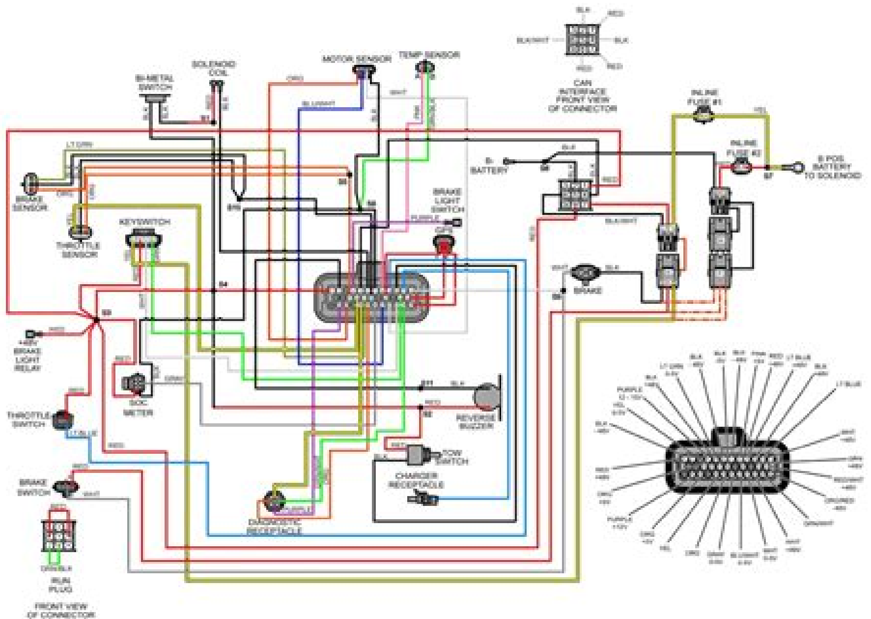
Fig. 29 Main Wiring Harness Diagram (after 23 January 2012)
