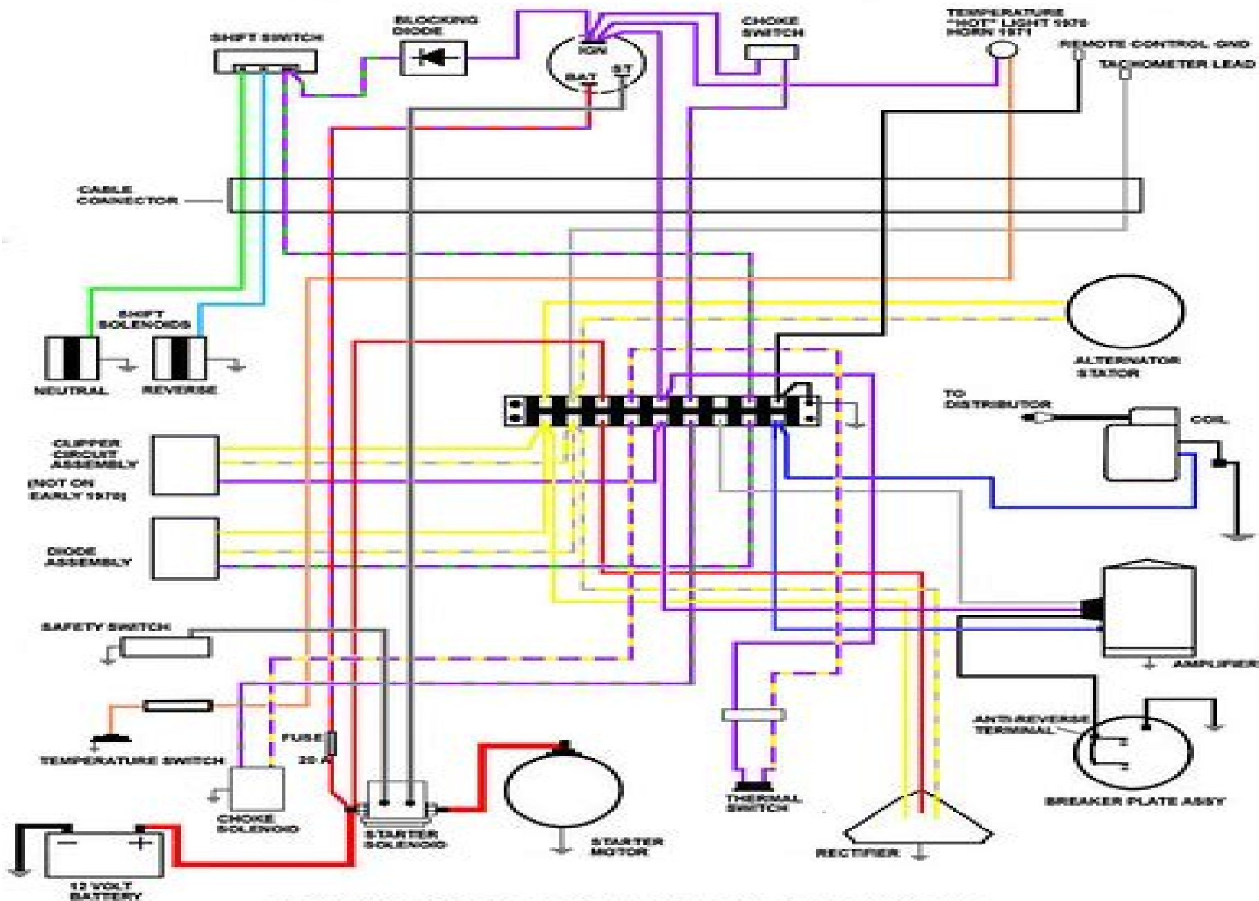
WIRING DIAGRAM 1970-71 60 HP 3 CYLINDER
