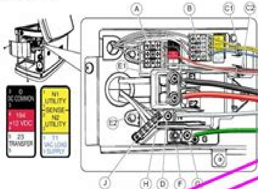
Figure 6-1. Electrical Wiring Connections
