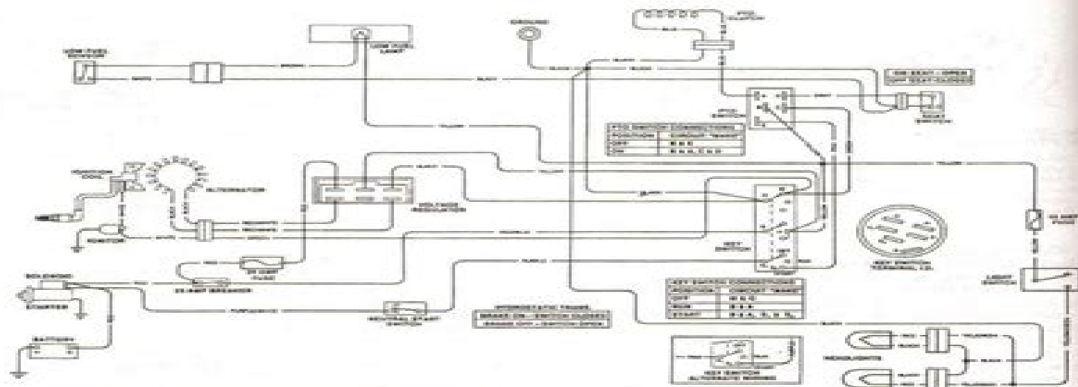
Fig. JD3-18—Electrical wiring diagram typical of Model 175.
