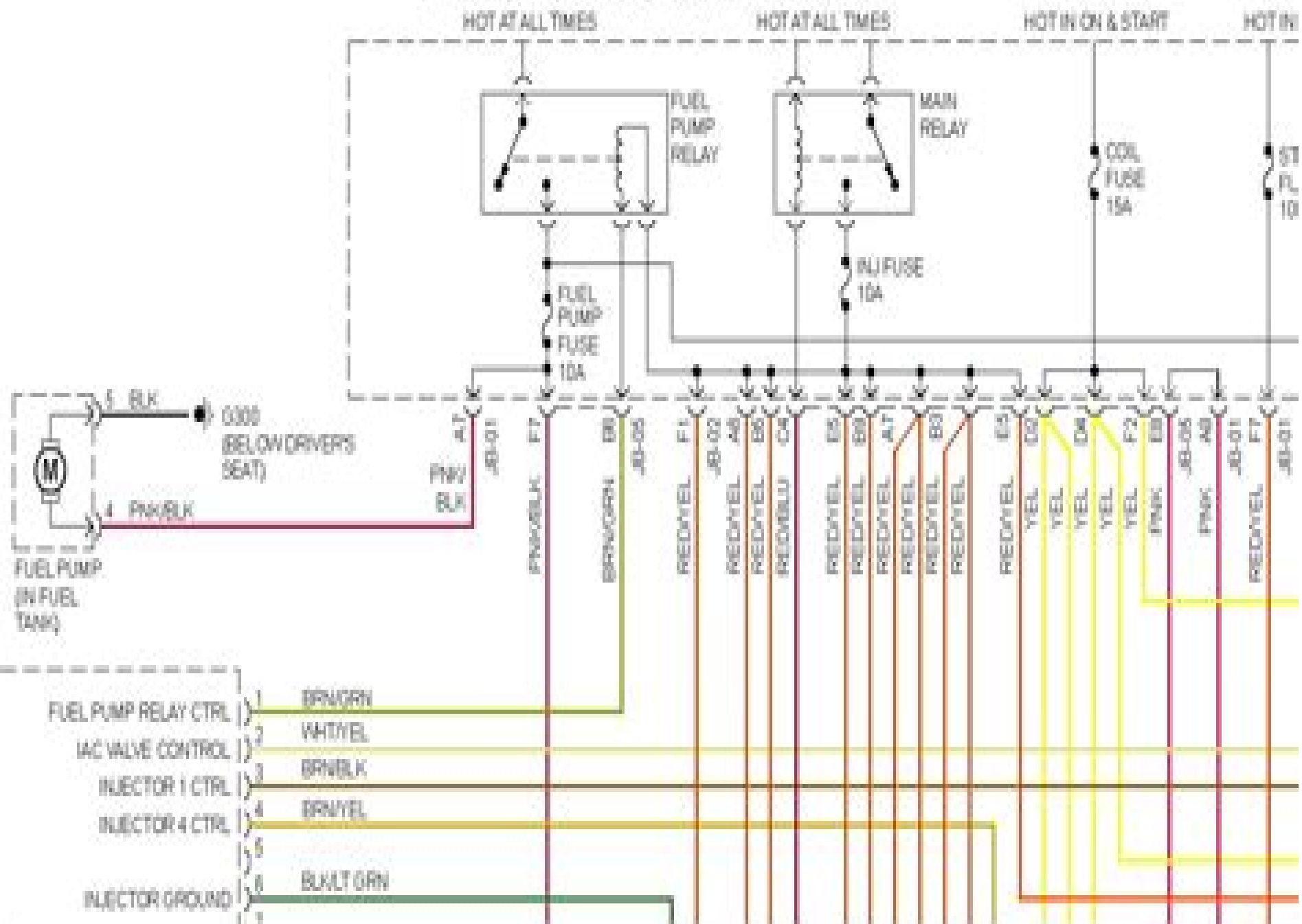
2001 Kia Sephia-Fig. 9: 1.8L, Engine Performance Circuits (1 of 3)
