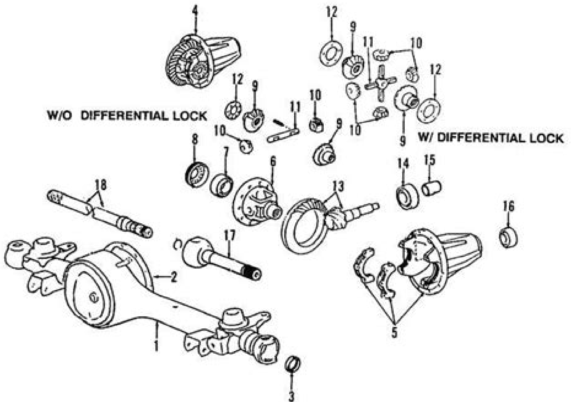
FRONT AXLE COMPONENTS-ONE PIECE HOUSING
