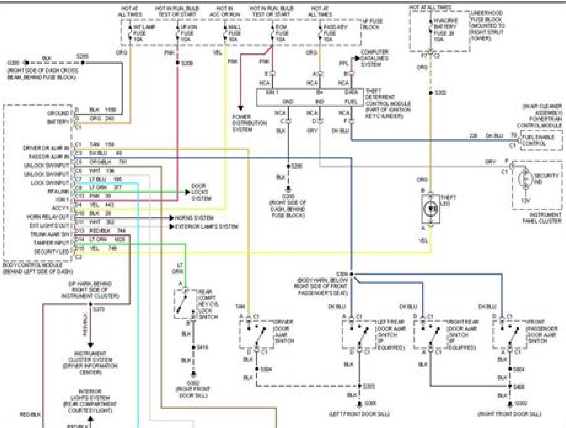
2002 Pontiac Grand Prix SE-fig. 4: Anti-theft Circuit
