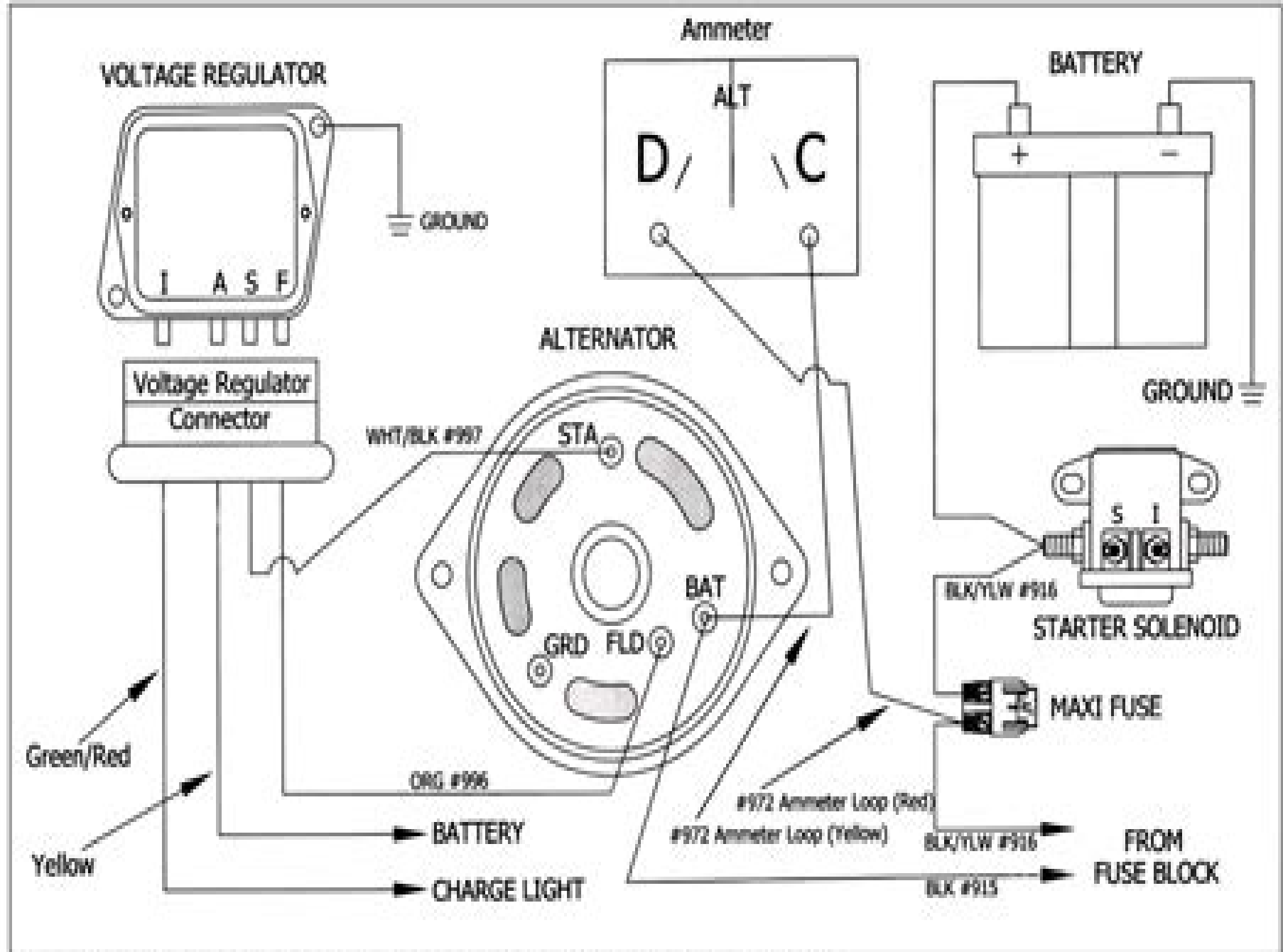
Figure 7-7 Alternator/Regulator/Solenoid Connections
