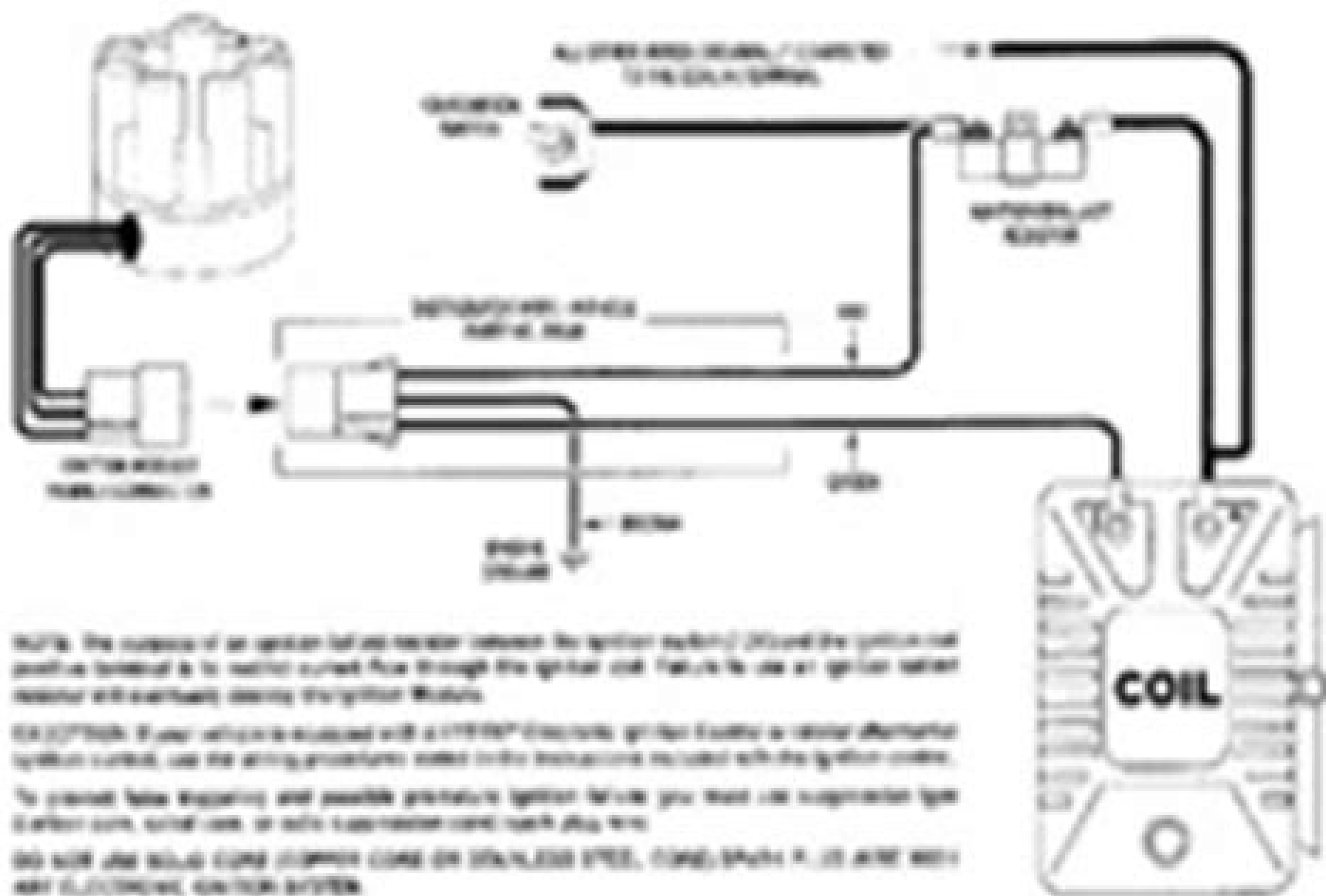
FIGURE 1 IGNITER WIRING DIAGRAM USING BALLAST RESISTOR
