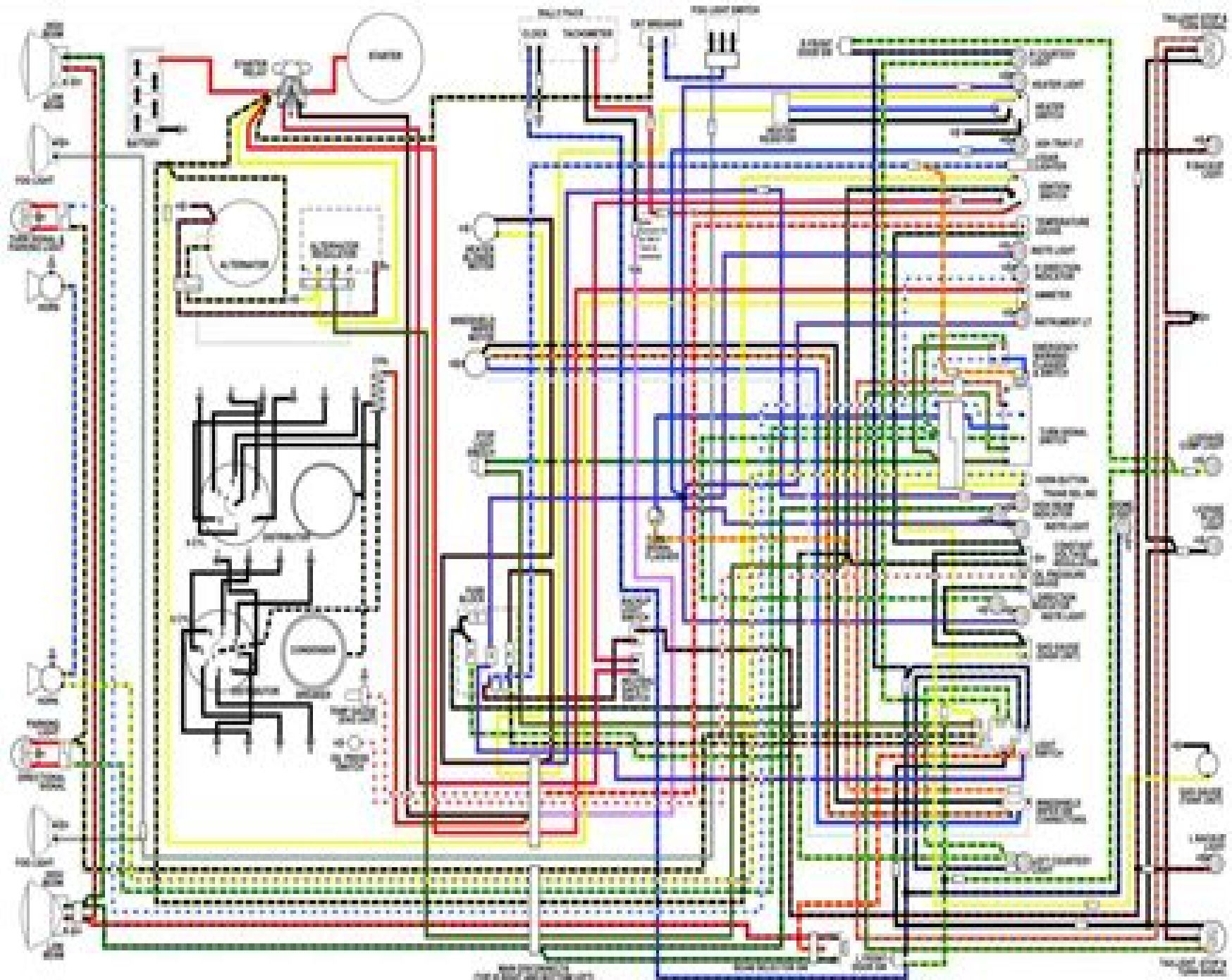
1966 MUSTANG CIRCUIT DIAGRAM (CLASSIC)
