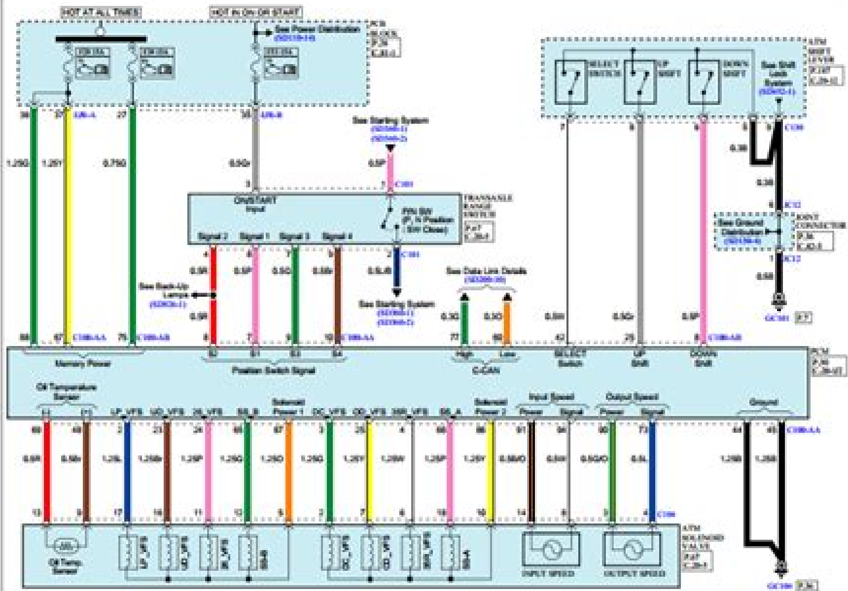
Automatic Transaxle Control System (G4NA : NU 2.0L MPI) (1)
