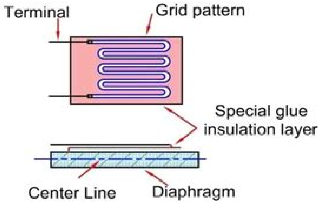
Grid configuration on the diaphragm
