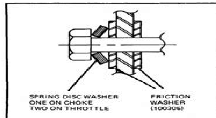
Fig. 1-1 Control Friction
