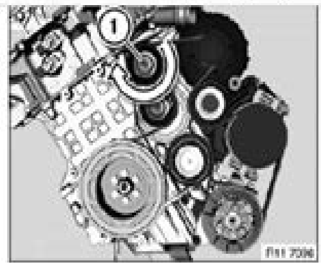
Fig. 168: Identifying Tensioning Pulley
