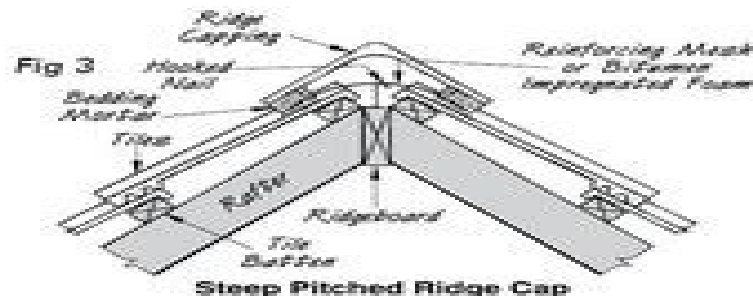
Steep Pitched Ridge Cap
