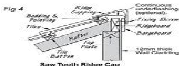
Saw Tooth Ridge Cap
