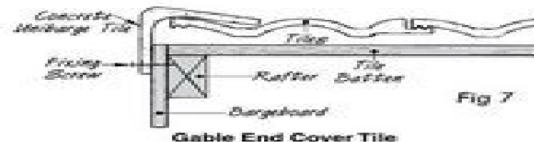
Gable End Cover Tile
