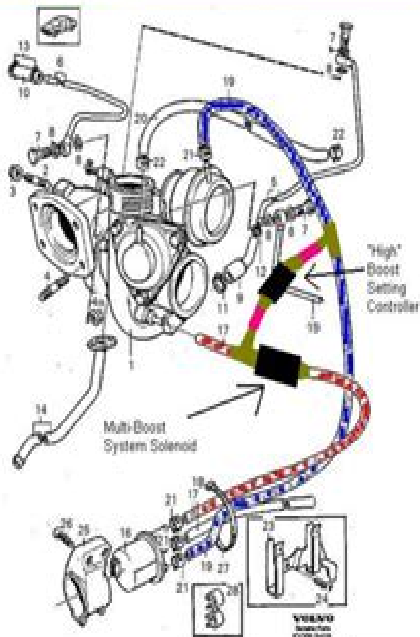
Turbocharger with connecting parts, SCYL 1000.
