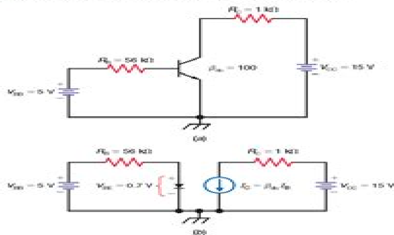
Figure 28-12 Base bias. (a) Circuit. (b) DC equivalent circuit.
