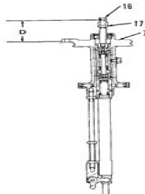
Fig. S218-32—Cross-sectional view of shift assembly. Distance (D) between housing (7) and center of hole in connector (16) with shift assembly in the neutral position, should be 46 mm (1.81 in.) on long shaft models and 173 mm (6.81 in.) on extra long shaft models. Tighten nut (17) securely.
