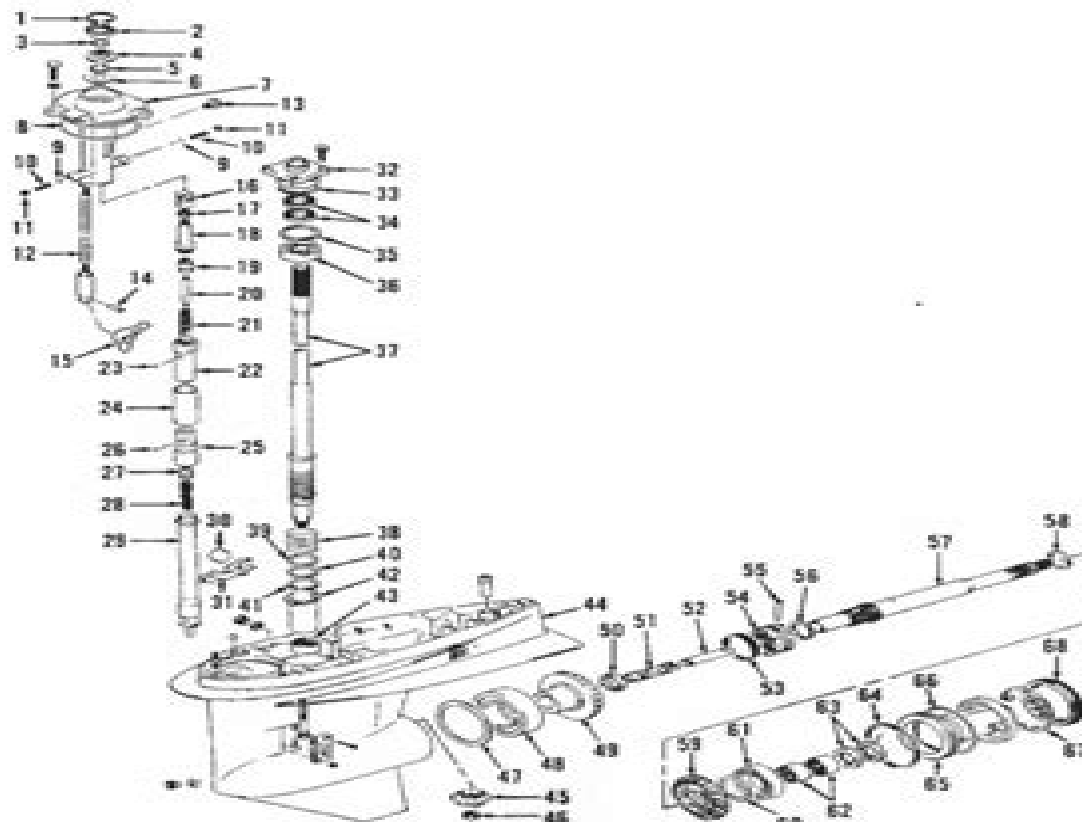
Fig. S218-31—Exploded view of lower unit gearcase assembly.
