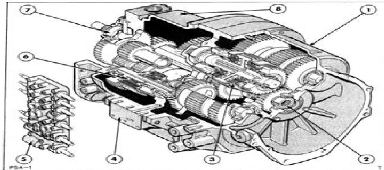
Figure 1 Mechanical Components of the powershift Transmission
