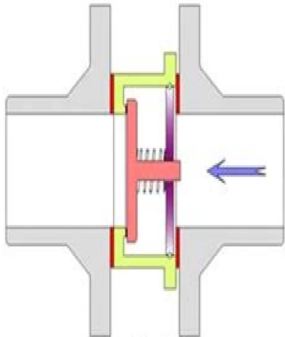
Close Position Reverse Flow
