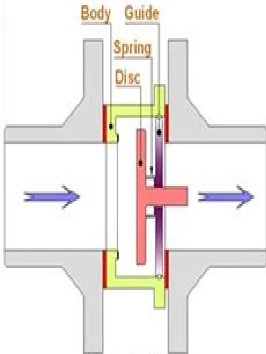
Open Position Forward Flow
