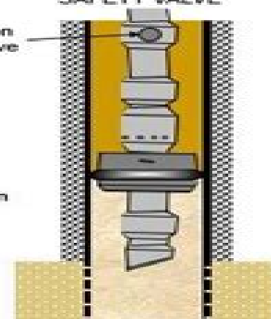
PACKER WITH NIPPLES, SLIDING SLEEVE AND SAFETY VALVE
