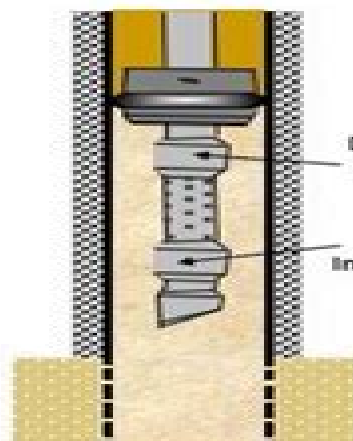
PACKER WITH PERFORATED TAIL PIPE
