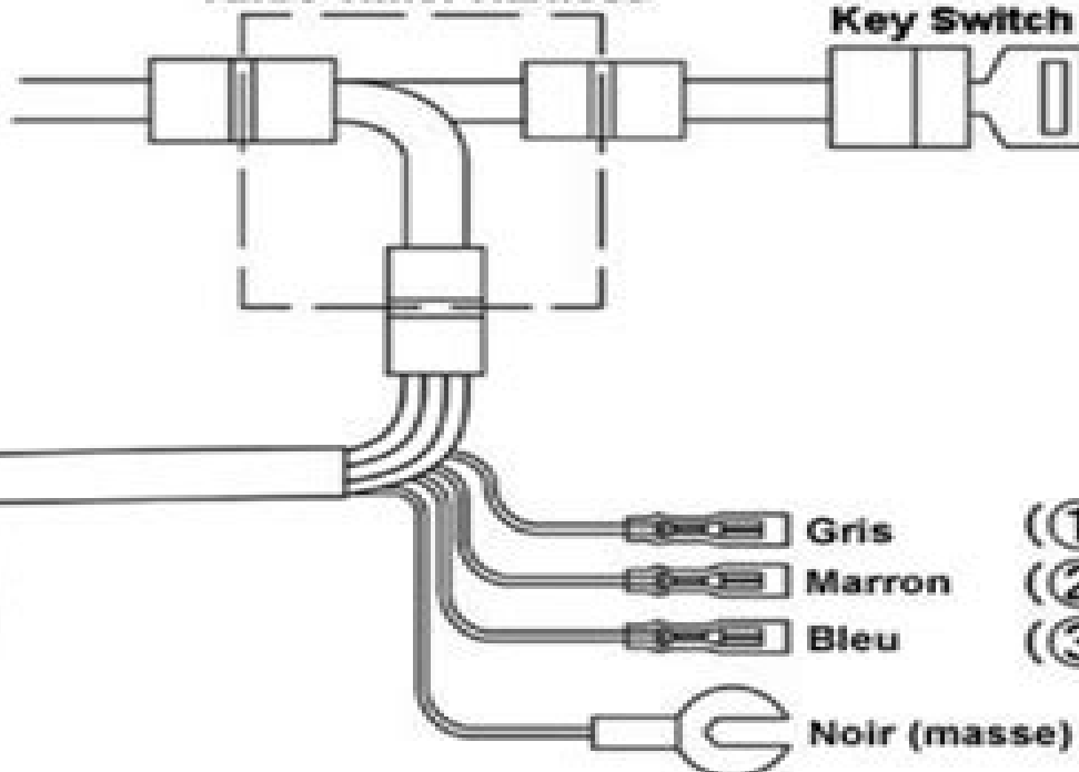
Turbo Timer Harness
