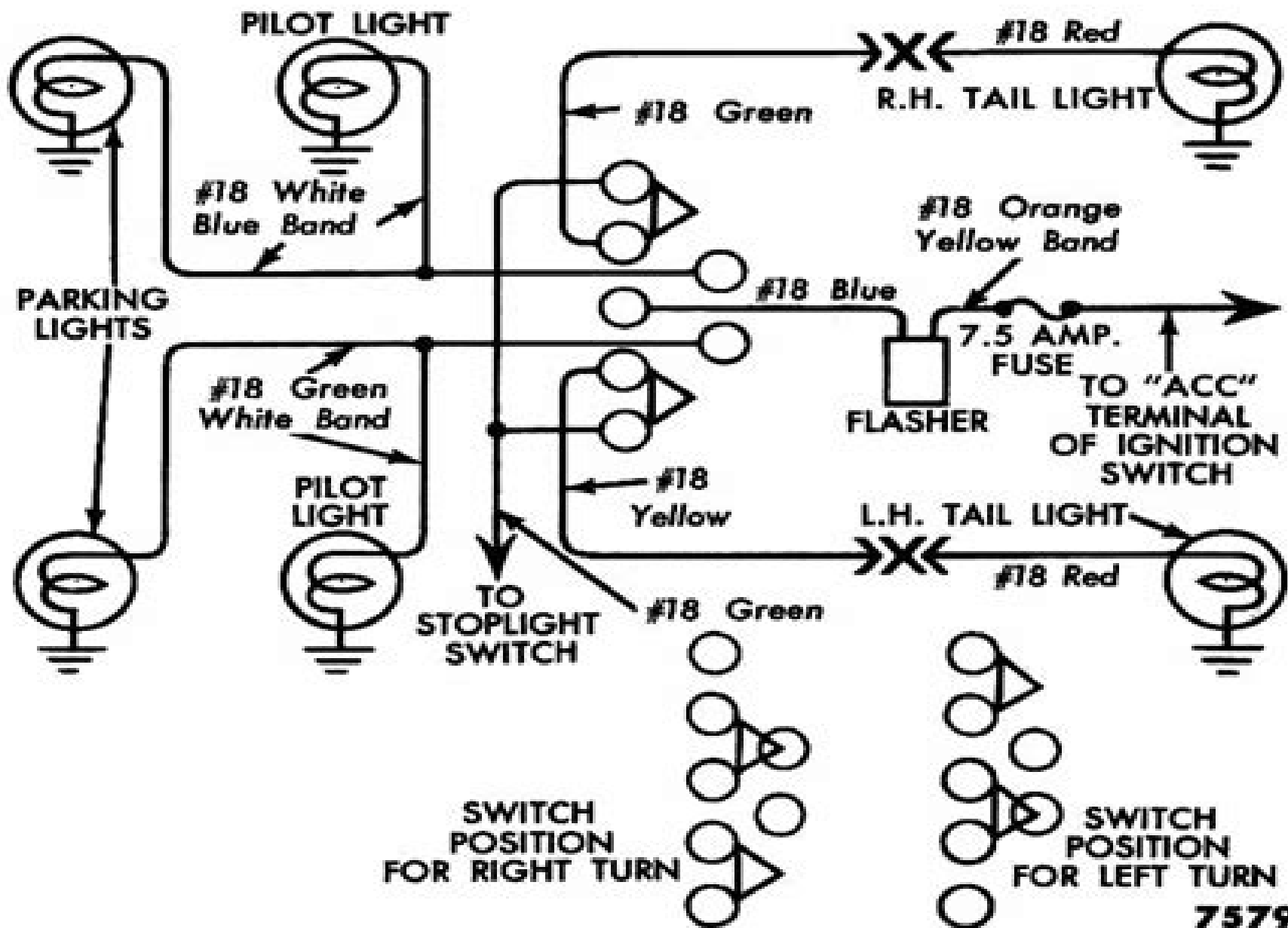
Fig. 1—Turn Signal Schematic Diagram
