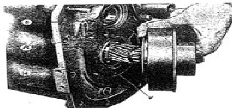
Fig. 99. - Assembling of epicyclic reduction gear on gearbox secondary shaft.
