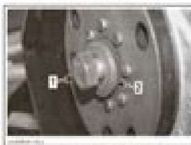
FIGURE 2 DRIVE PULLEY REMOVAL STEPS 1. Drive pulley removal screw 2. Conical spring washer
