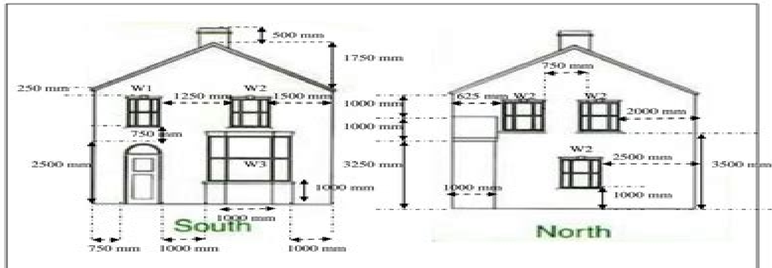
Fig 5.1 Front and back elevations
