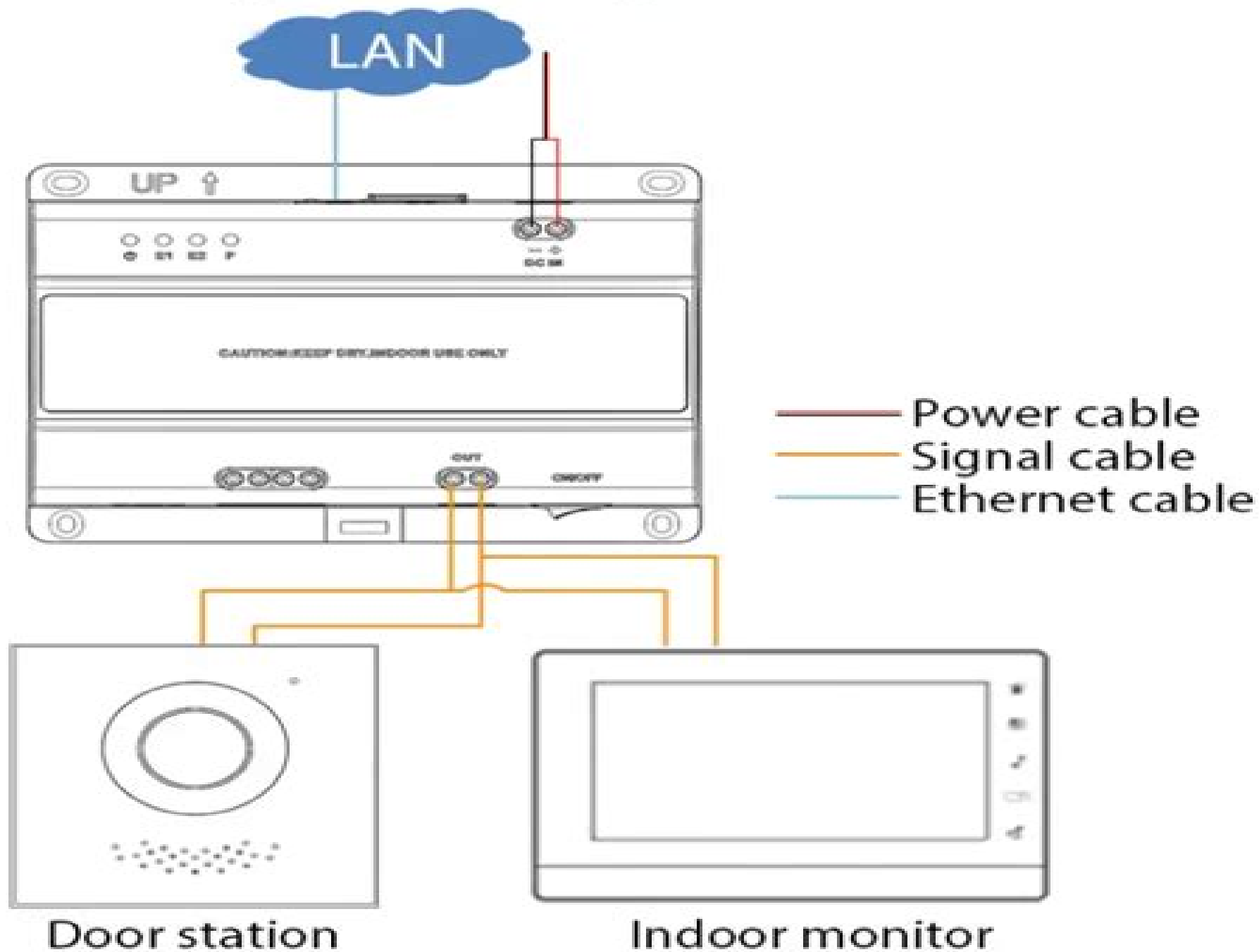
Figure 1-1 Villa network diagram
