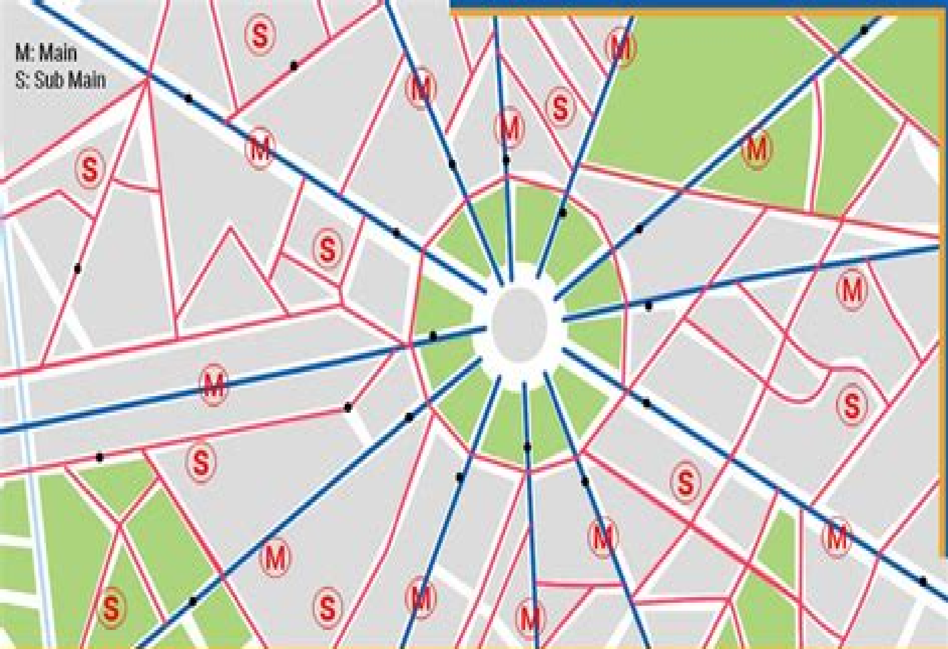
Layout of Water Distribution System
