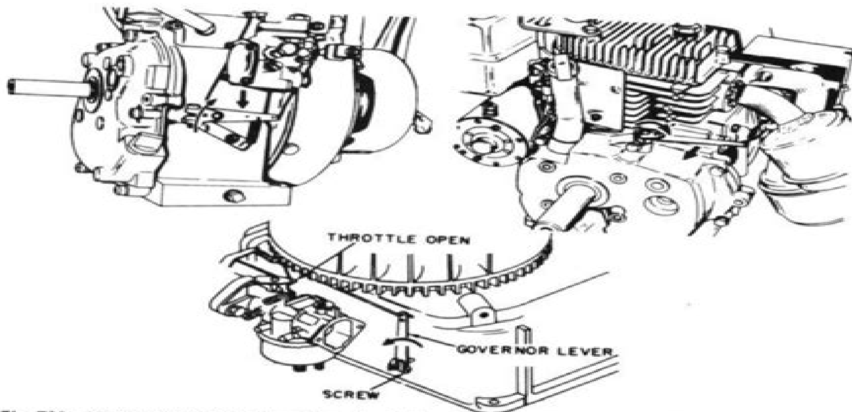
Fig. T28— Views showing location of mechanical governor lever and direction to turn when adjusting position on governor shaft.
