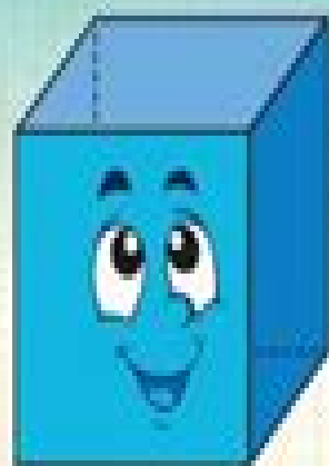
cube
