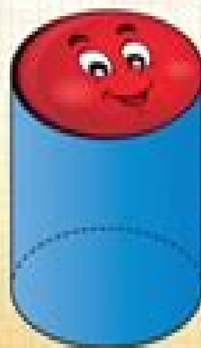
cylinder
