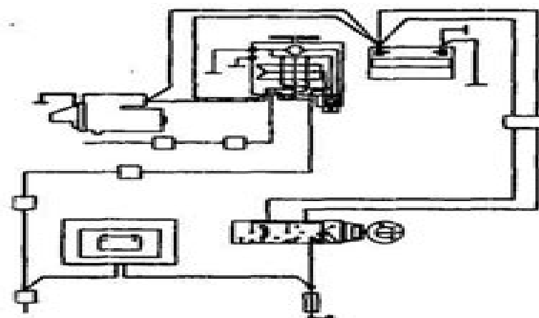
Alternator charging
