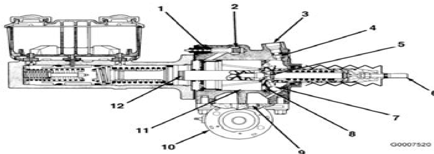
Figure 497 Hydraulic boost malfunction – Normal brake application
