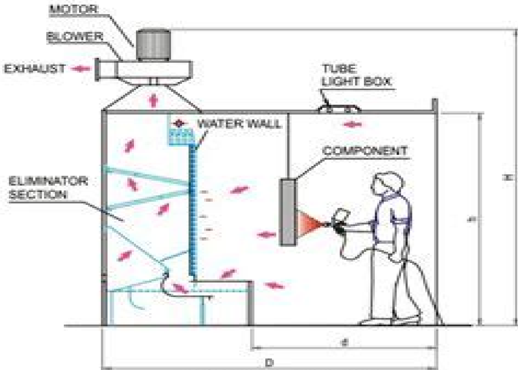
G.A. - Water Wash Paint Booth
