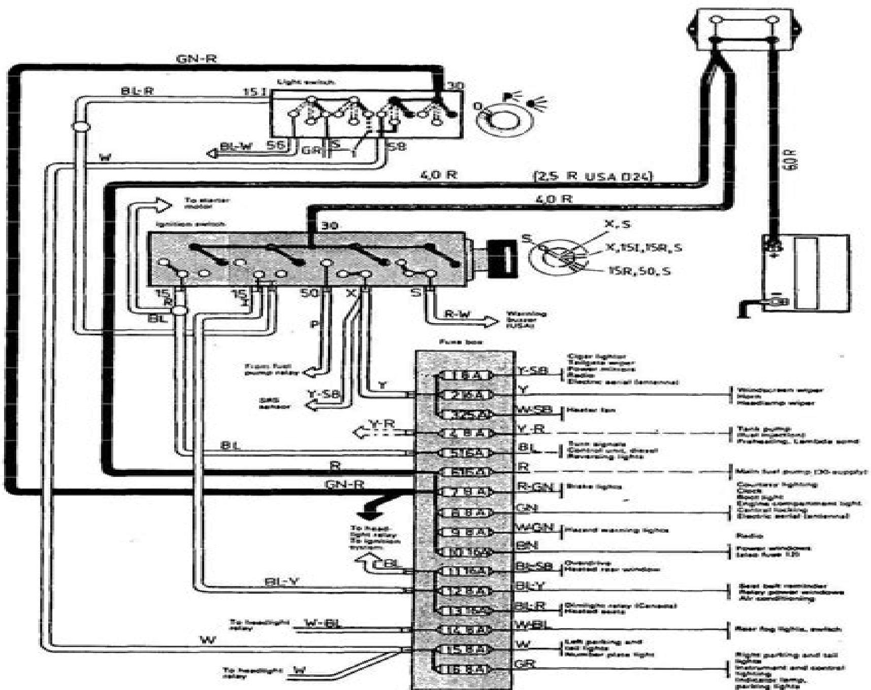
Fuse Panel. 240
