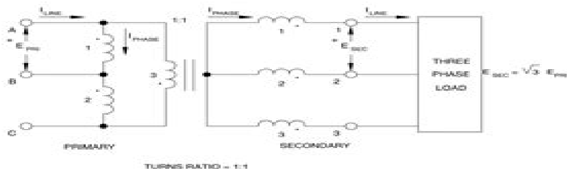
Figure 9-8. Three-phase delta-wye configuration.
